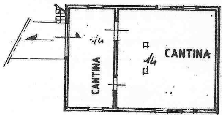
PIANO SEMINTERRATO H=2.37
